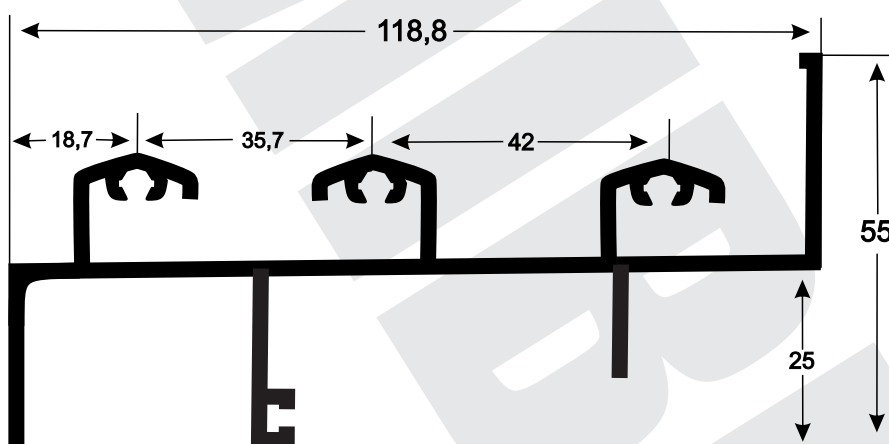
E-345 1,582 kg/m
